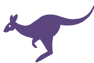
Kangaroo
