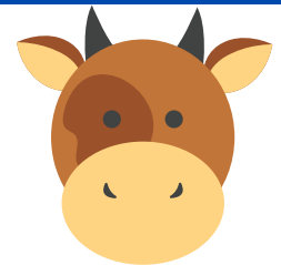
Cow
