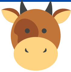
Cow
