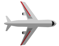
Plane
