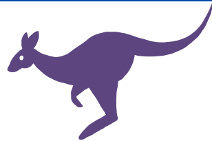
Kangaroo
