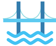
Bridge
